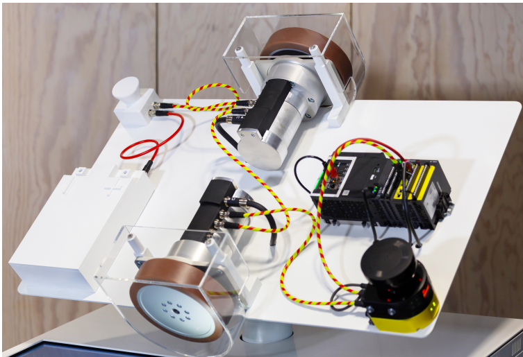
The robotics kit ROKIT and the automation toolkit ctrlX AUTOMATION from Bosch Rexroth simplify and accelerate the development and commissioning of automated guided vehicle systems. (Image source: Bosch Rexroth AG)
