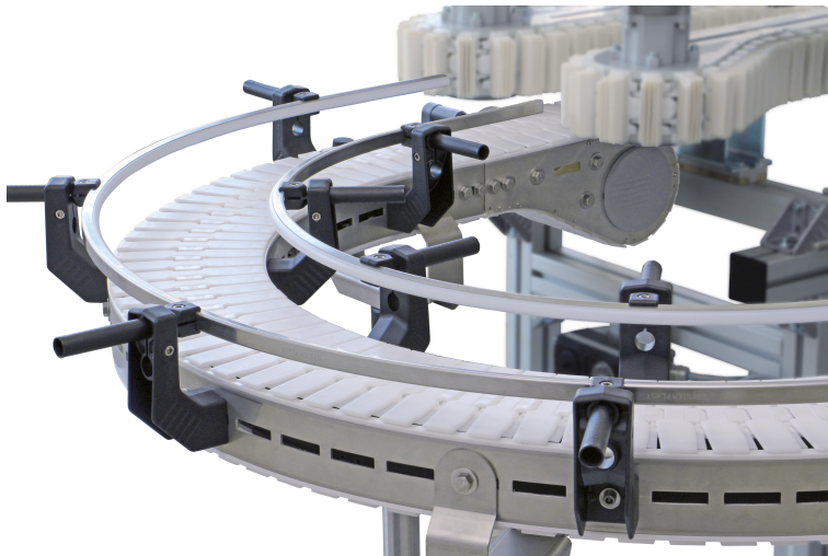
VarioFlow plus chain conveyor system from Bosch Rexroth with a stainless steel lateral guide (Image source: Bosch Rexroth AG)
