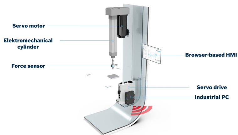
Image 2: Plug & produce with the Smart Function Kit: Examples for smart mechatronic solutions (Image source: Bosch Rexroth AG)
